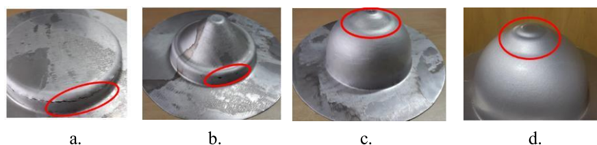
Gambar 9: Produk hasil: (a). single stage ; (b). multi-stage 2 tahap; (c). multi-stage 3 tahap; (d). multi-stage 4 tahap.
